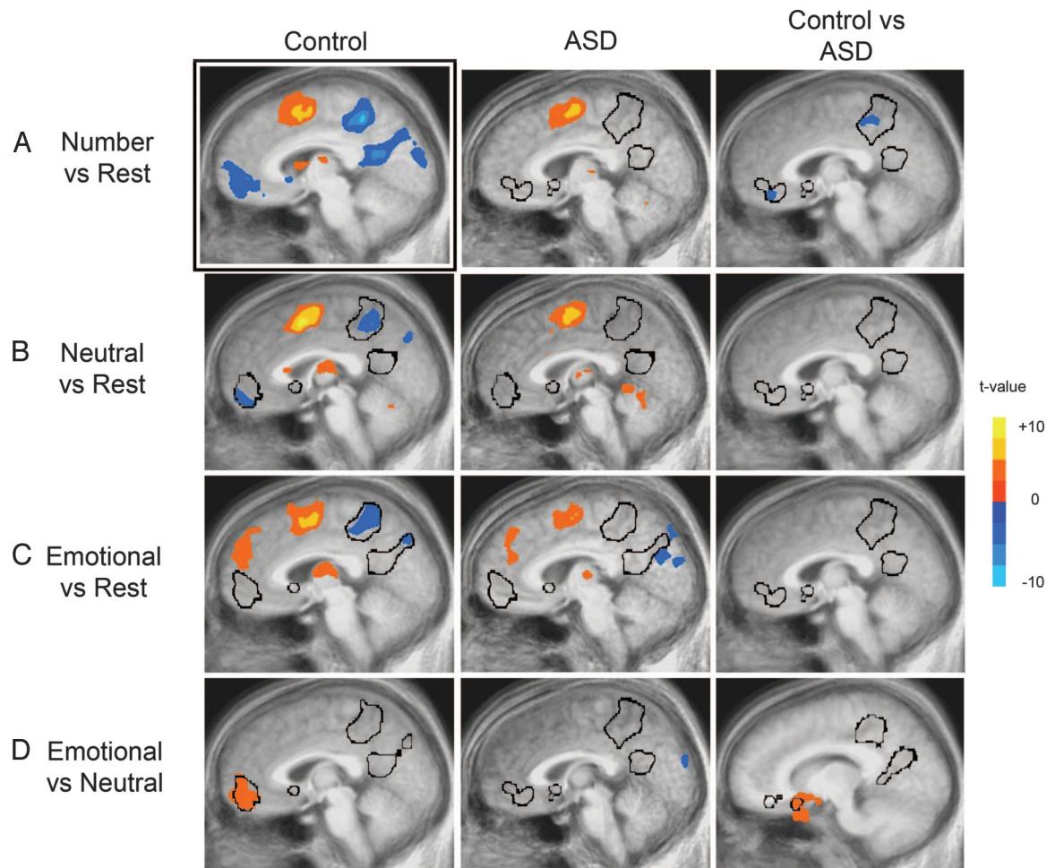
Fig. 1. Significant functional activity derived from group whole-brain analyses ( P < 0.01 , cluster corrected). t values are displayed, with negative t values representing deactivations. The black outlines correspond to the area of deactivation derived from the number vs. rest condition in controls (A Left) mapped onto the sagittal slices of the images shown. These outlines, which represent regions active during rest, highlight the presence or absence of activations or deactivations in each image. Each sagittal slice location differs slightly because each image was chosen to best represent the midline activity for each group and comparison. The comparisons shown are number vs. rest (A), neutral vs. rest (B), emotional vs. rest (C), and emotional vs. neutral (D).
